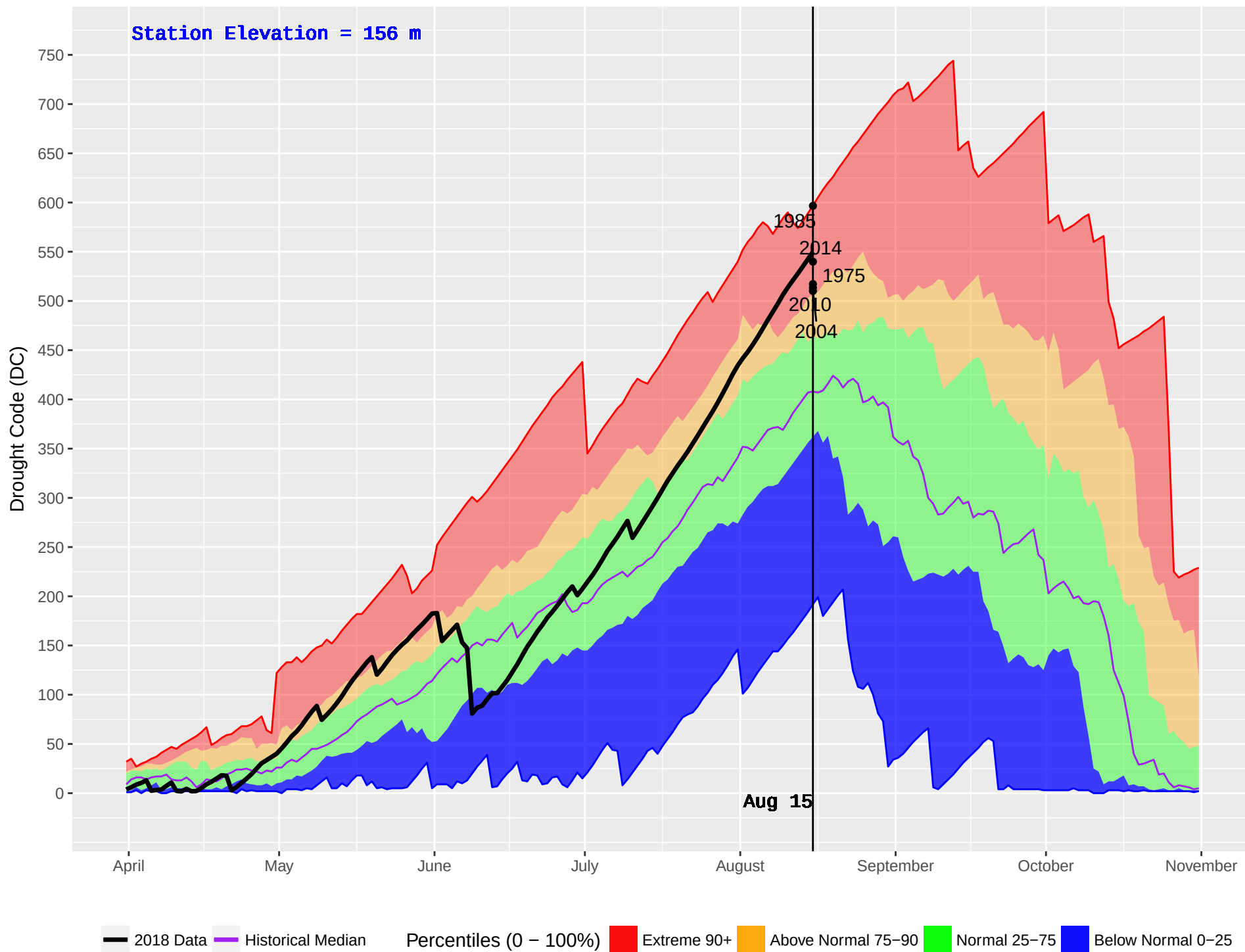
WOSS CAMP (21) : Historical (1970–2016) and Current (2018) Daily Drought Code (DC)
