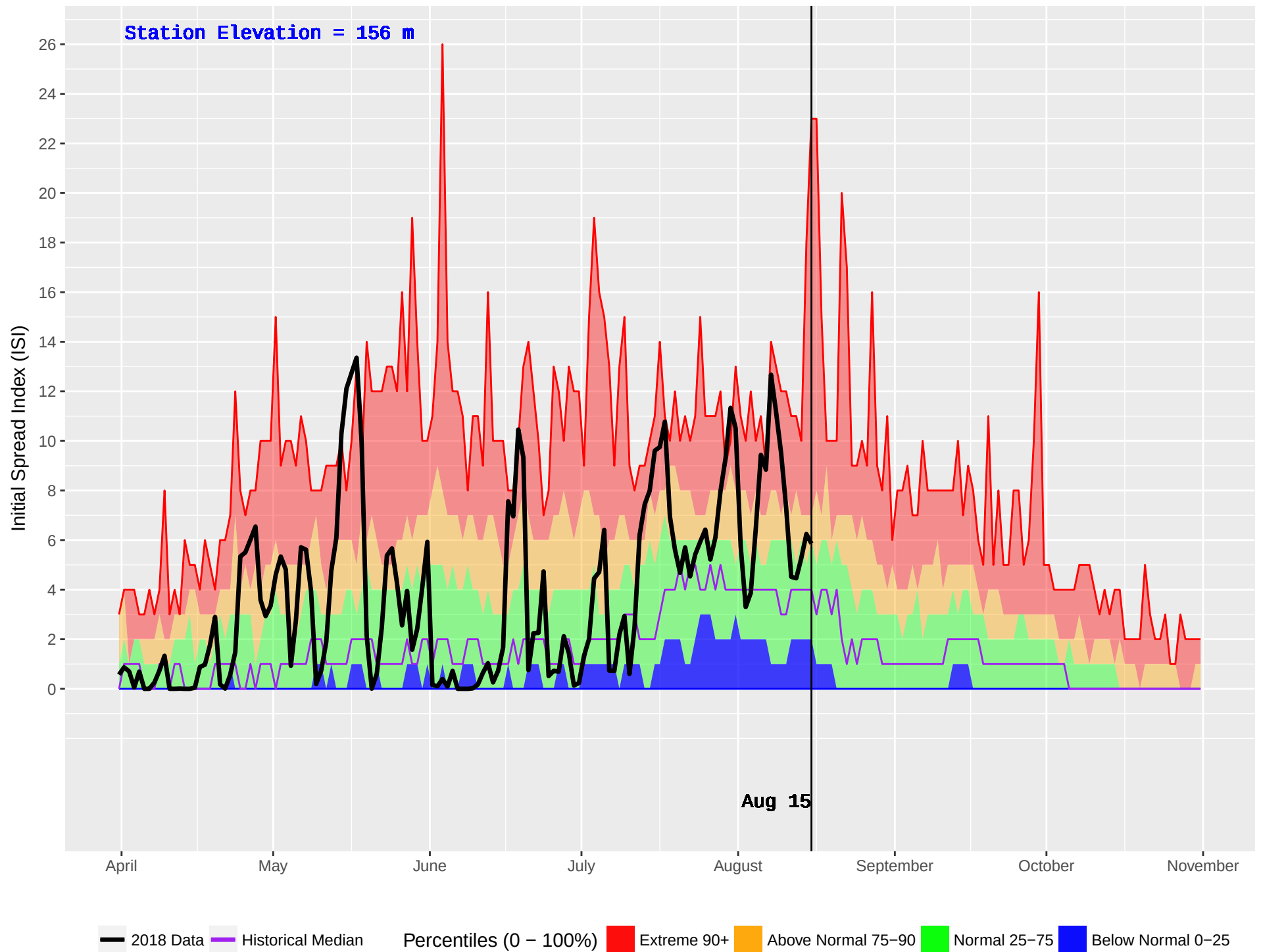
WOSS CAMP (21) : Historical (1970–2016) and Current (2018) Daily Initial Spread Index (ISI)
