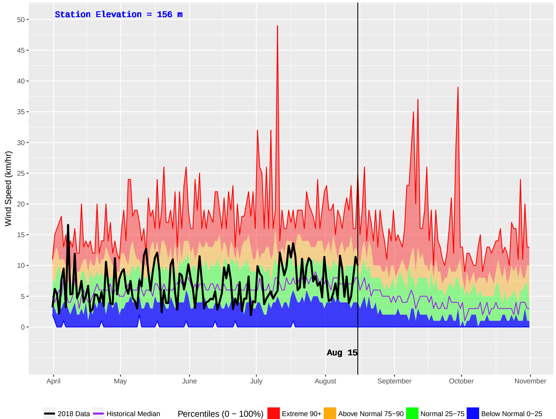
WOSS CAMP (21) : Historical (1970–2016) and Current (2018) Daily Wind Speed
